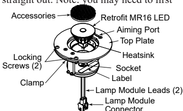
Retrofit MR16 LED Lamp Module
