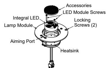
Integral LED Lamp Module
